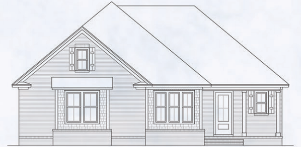
ELEVATION C
