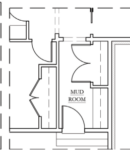
MUD ROOM W/DROP ZONE CABINETS
