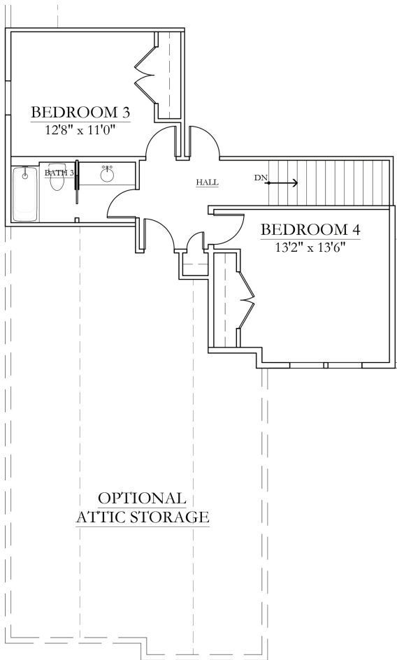
SECOND FLOOR - OPTION A 2,782 SQ FT
